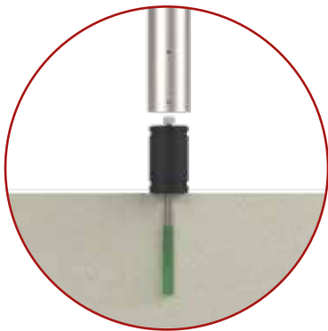
Bollard is fixed below ground using a nylon sleeve, chemical capsule & threaded stud
